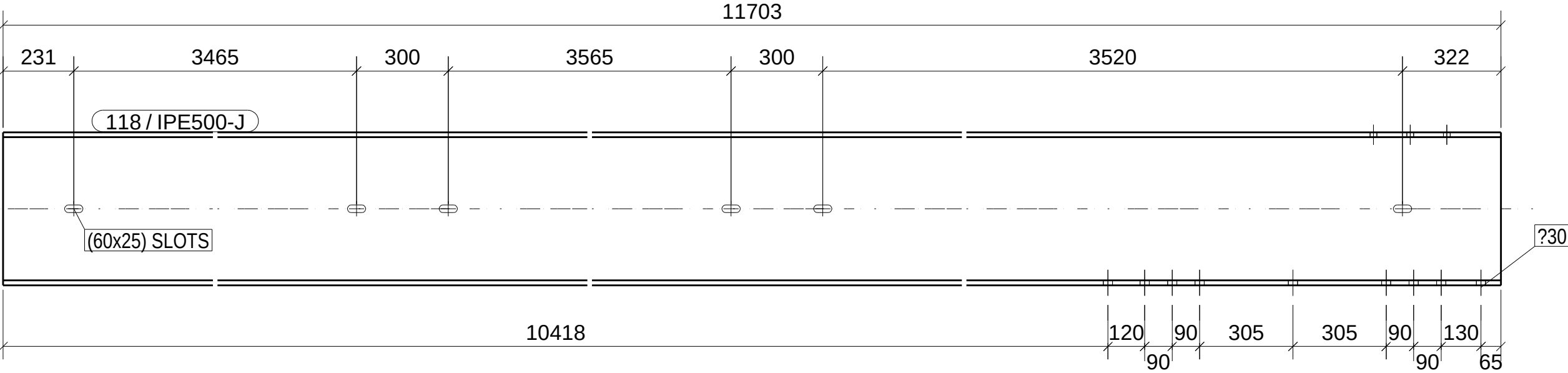
FRONT VIEW
